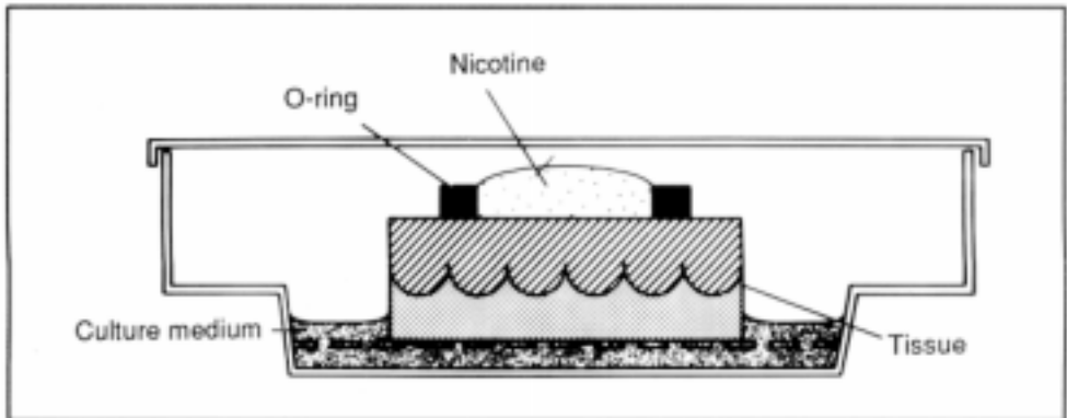
Figure 1 The model used to expose oral mucosa to topical nicotine
