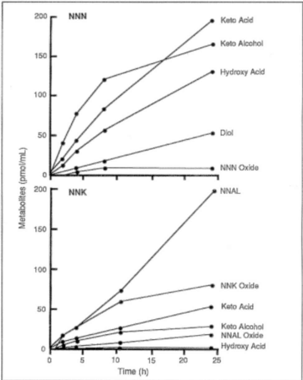
Figure 2 Formation of NNK and NNN metabolites by cultured rat oral tissue as a function of time
