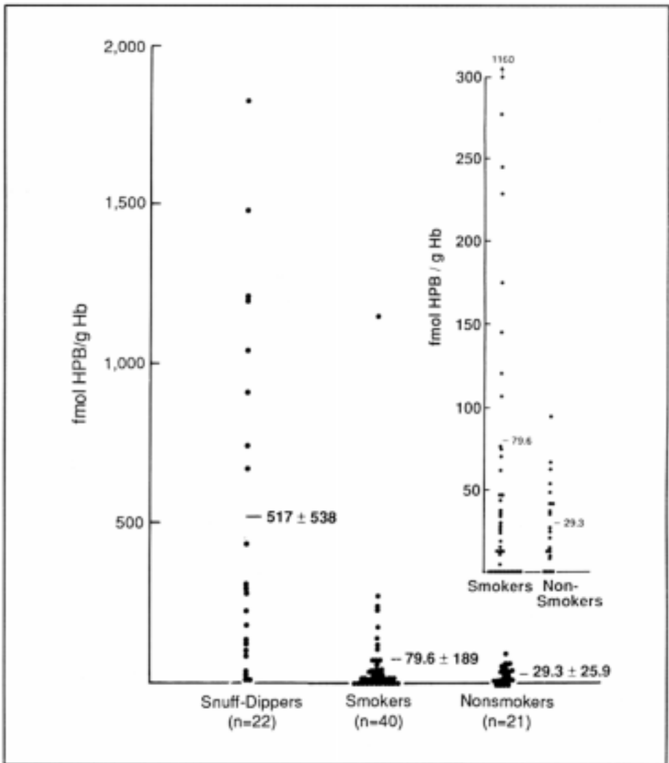
Figure 5 Levels of HPB released from hemoglobin of snuff dippers, smokers, and nonsmokers
