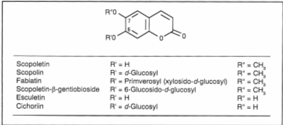
Figure 2 Coumarins in tobacco
