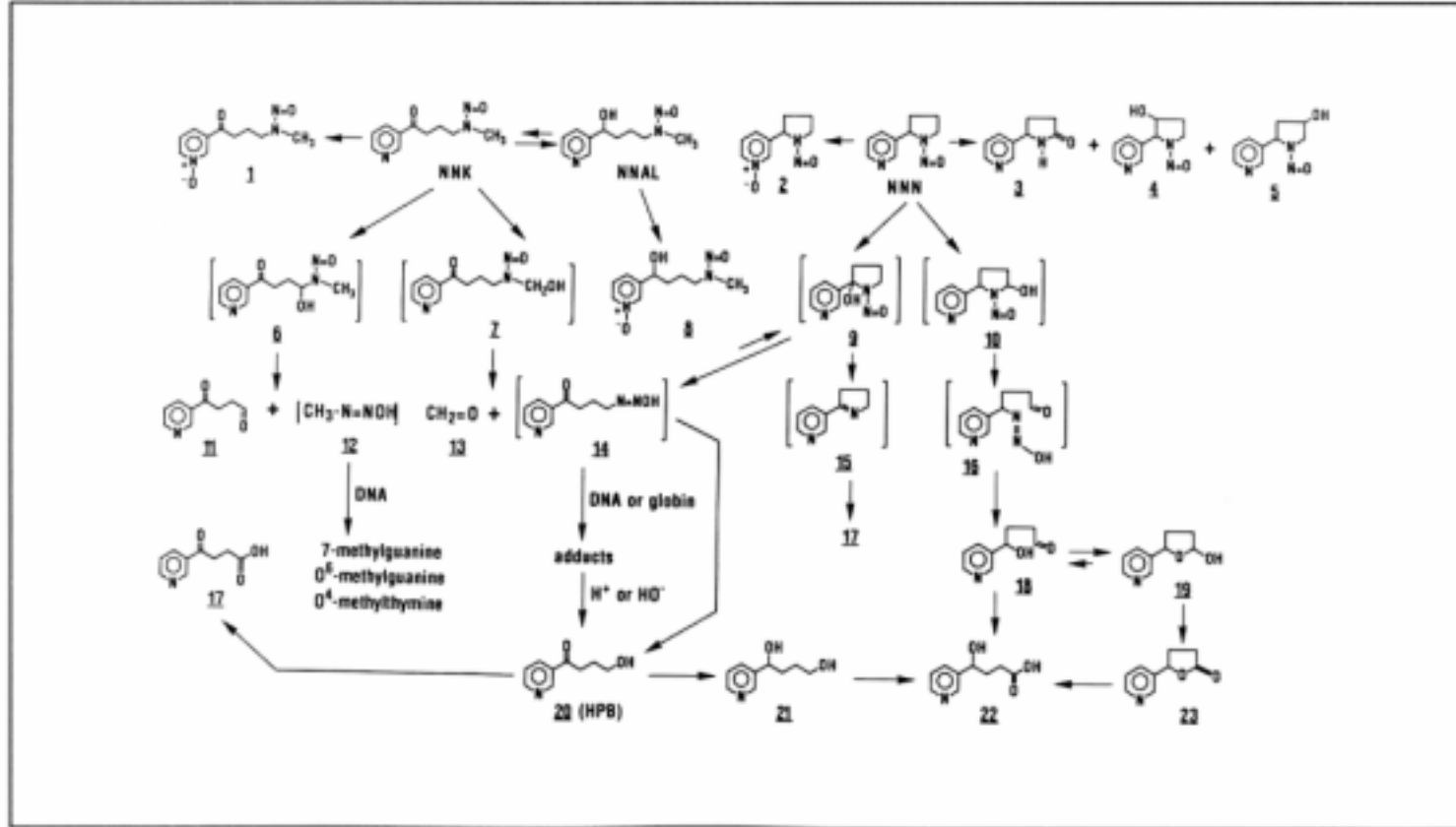
Figure 1 Metabolic pathways of NNK and NNN in rodents
